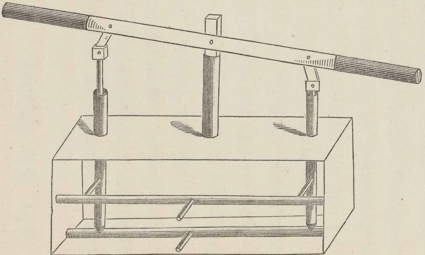
VIEW OF THE DOUBLE ACTING FORCE PUMP, WITH ONE SIDE OF THE BOX REMOVED
